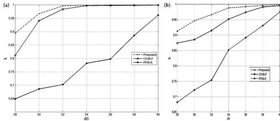
Figure 6. Change detection performance comparisons of various algorithms against different levels of noise. (a) Result on Ottawa image and (b) result on Yellow River Estuary image.
