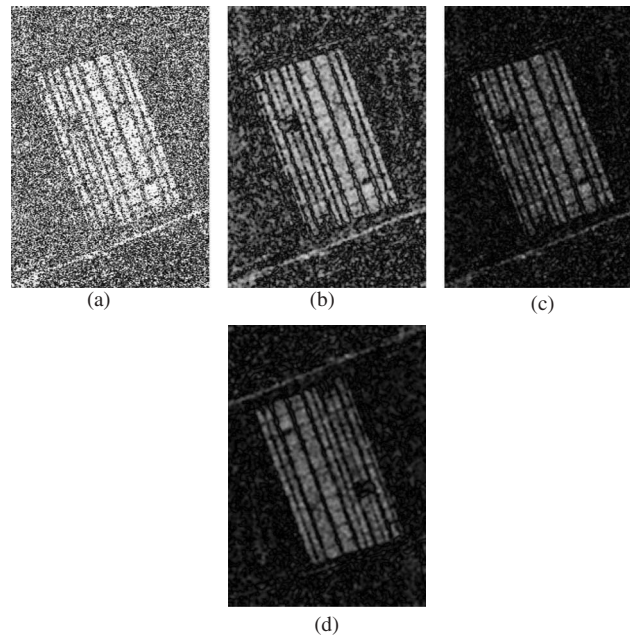
Figure 3. The various difference maps (a) log-ratio difference map based on source image (b) mean ratio difference map based on source image (c) log-ratio difference map based on logarithmic domain (d) mean ratio difference map based on logarithmic domain.
